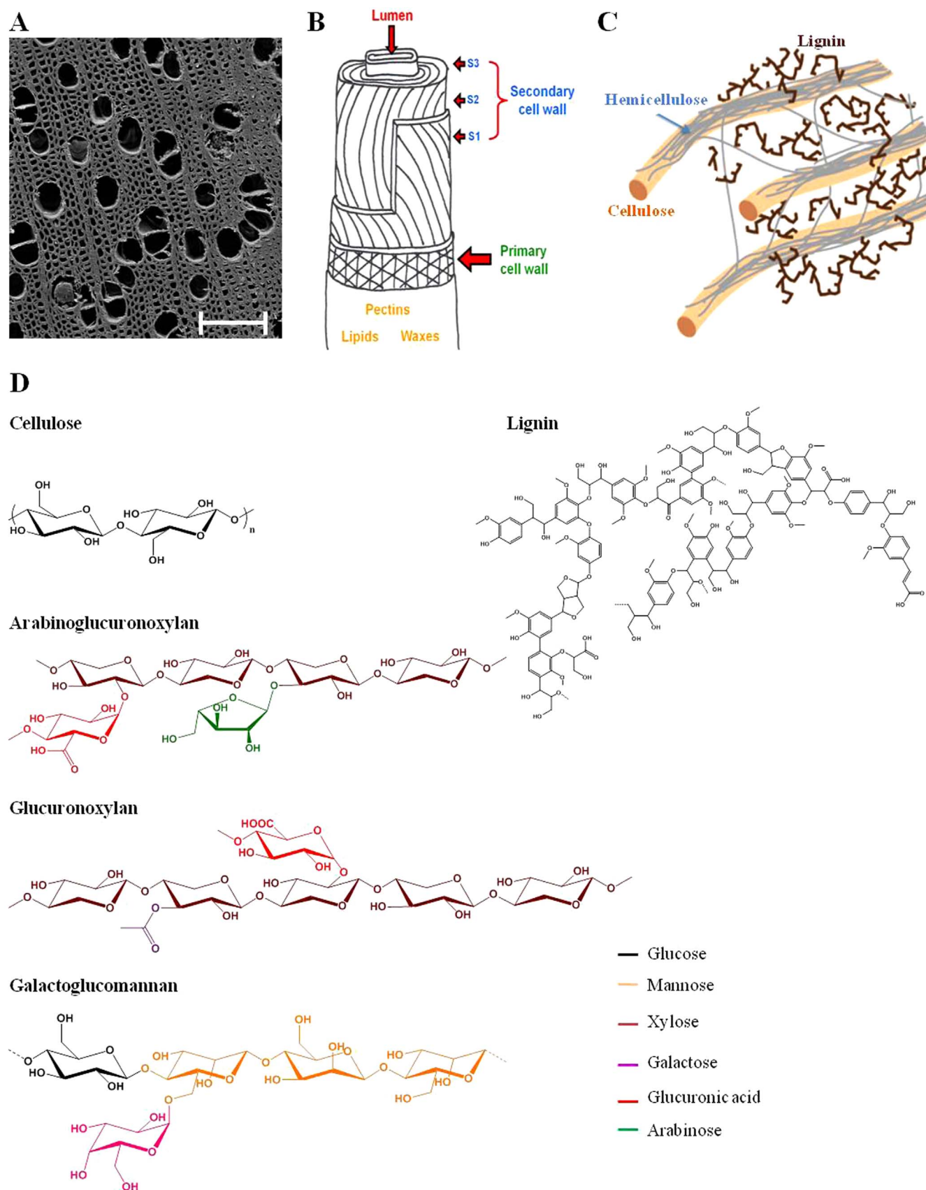
Fig. 5. Diagrammatic illustration of the framework of wood cell wall. A, Anatomical structure of willow wood (Scale bar=100 μm); B, Cell wall structural organization; C, Cell wall polymer interactions in secondary cell wall of hardwood; D, Secondary cell wall polysaccharide structures different colors show different sugars.
