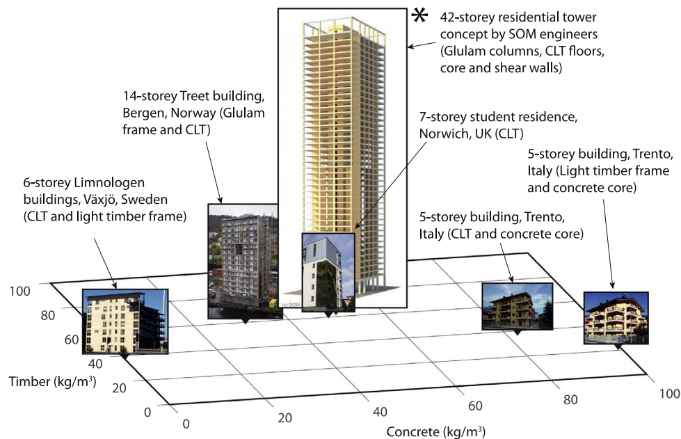
Fig. 23. Material usage, in terms of mass, in multi-storey timber buildings. The horizontal axes show the mass of timber or concrete used per \text{m}^3 of each building. The size of the images indicates the height of each of the six case-study buildings investigated – the building indicated by * is a concept, and has not been constructed (image by SOM [103]).
