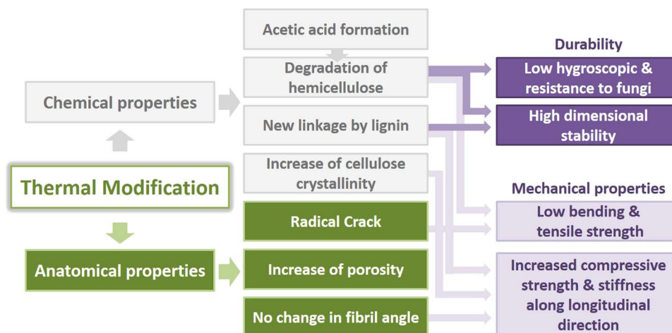
Fig. 19. Property changes involved in the thermal modification.
